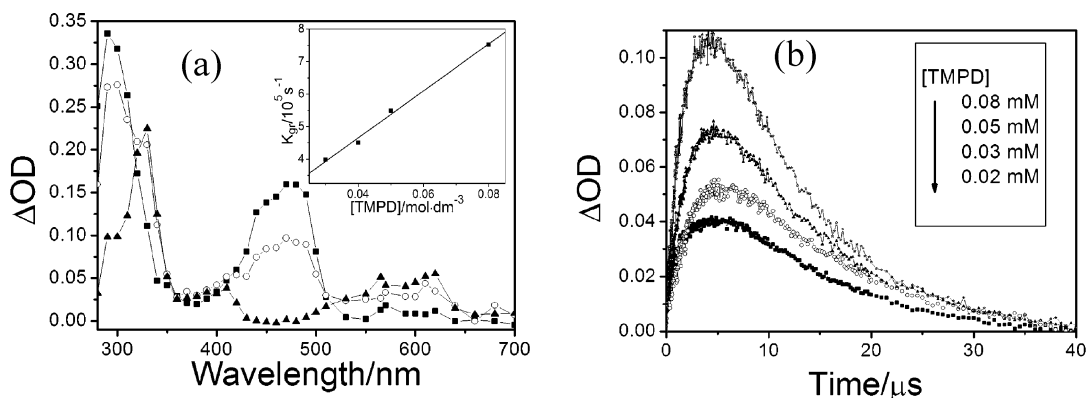
Figure 3. (a) Transient absorption spectra recorded at (■) 0.1, (○) 1, and (▲) 5 \mu\text{s} after 355 nm excitation of the \text{N}_2 -saturated neat MeCN containing 1 \times 10^{-4} \text{ mol}\cdot\text{dm}^{-3} DQ and 1 \times 10^{-4} \text{ mol}\cdot\text{dm}^{-3} TMPD. Inset: The first-order growth rate of \text{TMPD}^{*+} at 565 nm is plotted as a function of TMPD concentration. (b) Time profiles observed at 565 nm for \text{TMPD}^{*+} .
