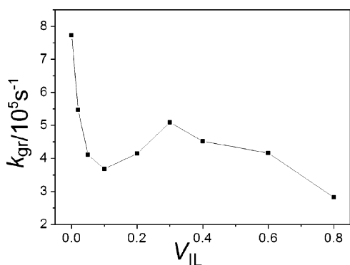
Figure 5. Dependence of the observed growth rate constant ( k_{\text{gr}} ) of \text{TMPD}^{*+} on the volume fraction of [bmim][PF 6 ]. ( V_{\text{IL}} = 0.1 corresponds to a mole fraction of about 0.027.)
