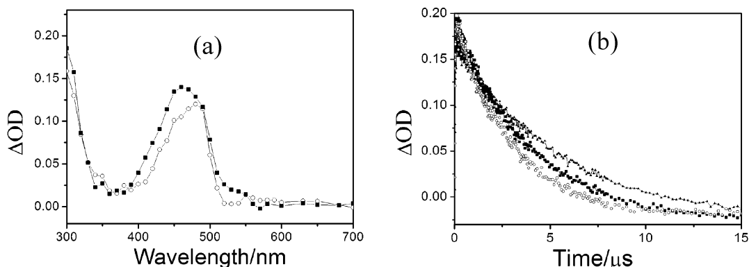
Figure 1. (a) Transient absorption spectra of {}^3\text{DQ}^* recorded at 0.1 \mu\text{s} after 355 nm laser excitation in a IL/MeCN solution containing 1 \times 10^{-4} \text{ mol}\cdot\text{dm}^{-3} DQ under \text{N}_2 . V_{\text{IL}} : (○) 0 and (■) 0.8. (b) Decay profiles monitored at 480 nm recorded in IL/MeCN mixed solutions in the presence of 1 \times 10^{-4} \text{ mol}\cdot\text{dm}^{-3} DQ under \text{N}_2 purging. V_{\text{IL}} : (middle) 0, (bottom) 0.2, (top) 0.8.
