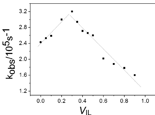
Figure 2. Dependence of the 3 DQ* decay rate constant ( k_{\text{obs}} ) at 480 nm on V_{\text{IL}} in mixed solutions. ( V_{\text{IL}} = 0.3 corresponds to a mole fraction of about 0.1.)
