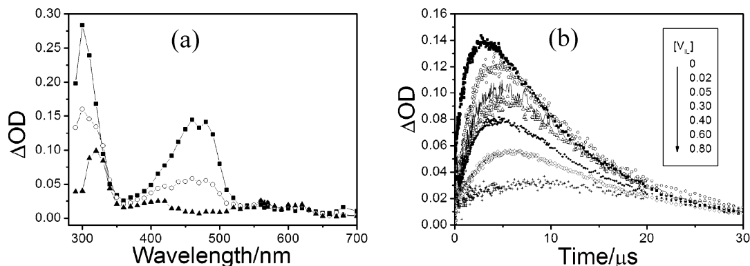
Figure 4. (a) Transient absorption spectra recorded at (■) 1, (○) 5, and (▲) 10 \mu\text{s} after 355 nm excitation for a \text{N}_2 -saturated IL/MeCN solution ( V_{\text{IL}} = 0.8 ) containing 1 \times 10^{-4} \text{ mol}\cdot\text{dm}^{-3} DQ and 1 \times 10^{-4} \text{ mol}\cdot\text{dm}^{-3} TMPD. (b) Time profiles of \text{TMPD}^{*+} observed at 565 nm for IL/MeCN solutions with different V_{\text{IL}} values.
